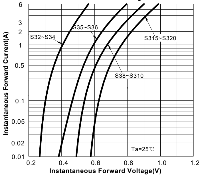
FIG3: Forward Voltage
